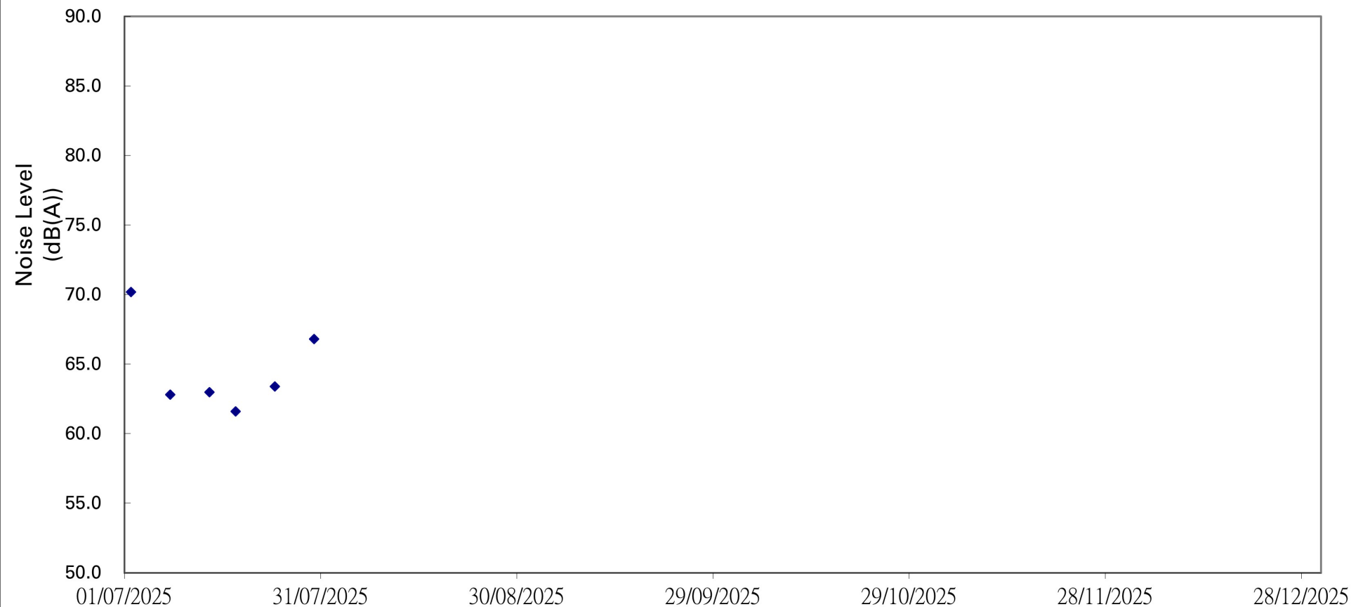
Noise Level (Leq 30 mins) dB(A) Vs Date for Location W-N18
